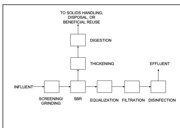
Figure 1: Process flow diagram for SBR
